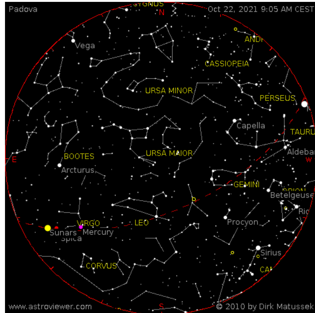
Sky map by AstroViewer [1]@ Get the HTML code [2] for this sky map
